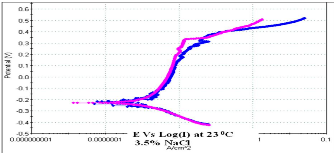
Blue line corresponds to 316L Pink line corresponds to J216L
